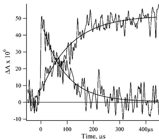
Figure 12. Kinetic traces for the growth of carbazole 9 (1241 \text{cm}^{-1} ) and the decay of azacycloheptatetraene 1f (1868 \text{cm}^{-1} ), obtained by TRIR spectroscopy after LFP of 1a in acetonitrile at ambient temperature.
